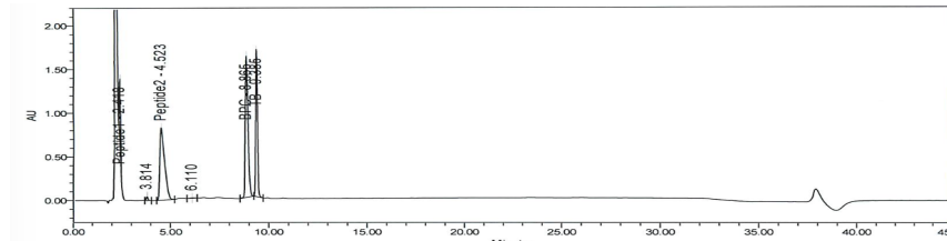
HPLC-MS Chromatogram
