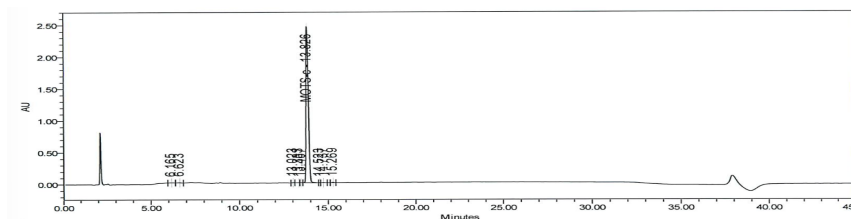
HPLC-MS Chromatogram
